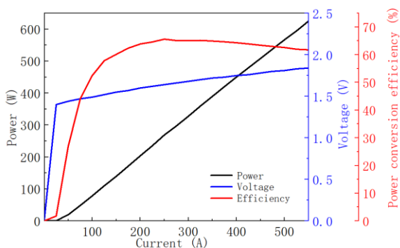
Power-Current-Voltage-Efficiency
